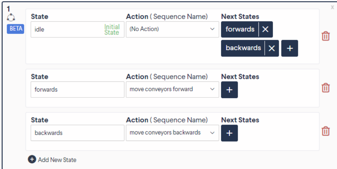
Figure 2: Simple State Machine in MachineLogic
